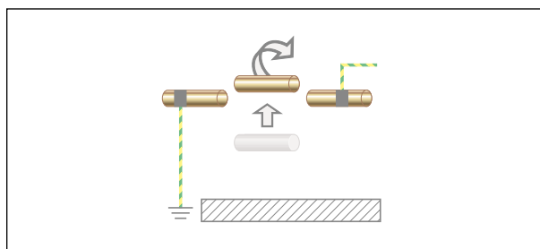
Fig. 7-14 Potential equalisation while replacing pipes
