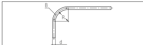
Fig. 6-6 Pipe bend
