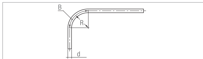
Fig. 7-15 Pipe bend
